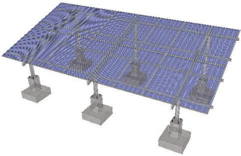
SOLAR STRUCTURE & PV PANEL
